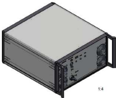
Controller (height = 184; width = 343; length = 375 core dimensions in mm )
